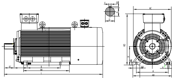
Figure 1 B3
