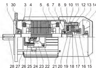
Figure 2 B5 63~112
