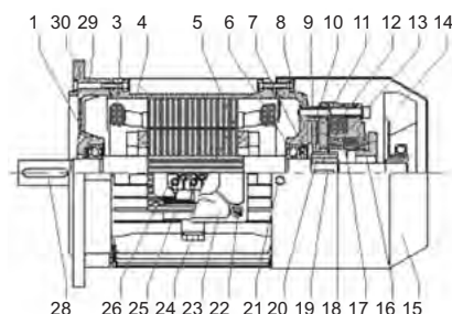
Figure 3 B5 132~160
