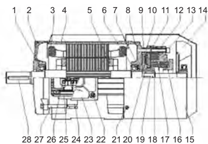
Figure 1 B5 63~160
