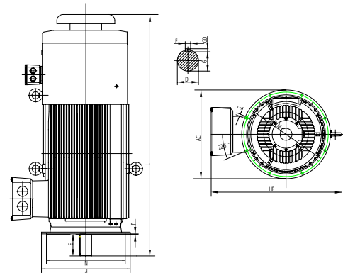
Figure 3 B5
